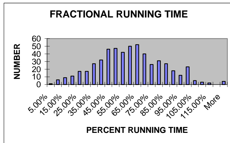
Figure 3. Estimated Refrigerator Fractional Run Time or Capacity Factor.
