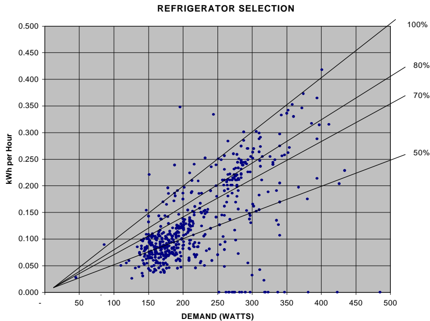
Figure 4. Refrigerator Selection Criteria Demand verses Usage.
